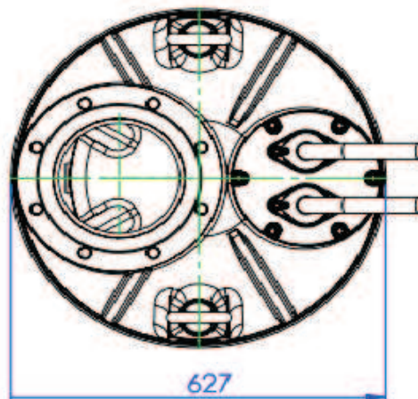
VIEW CK
