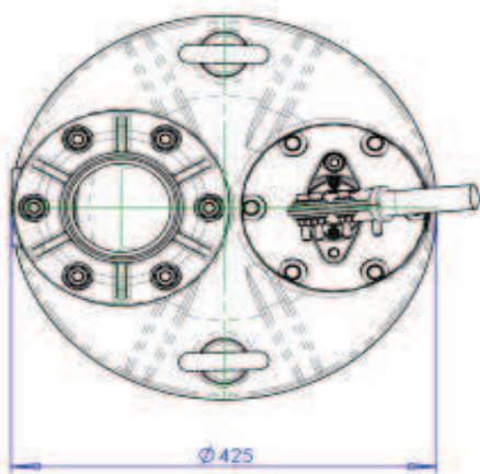
VIEW CK
