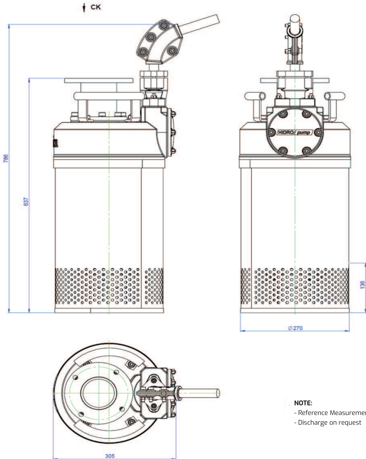
VIEW CK
