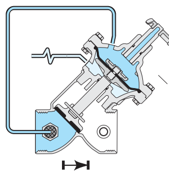
Normally Closed Valve with Hydraulic Power Opening
