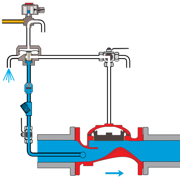
Valve Open (operating condition)
