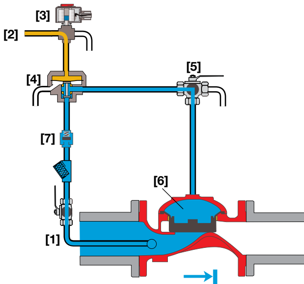
Valve Closed (set position)
