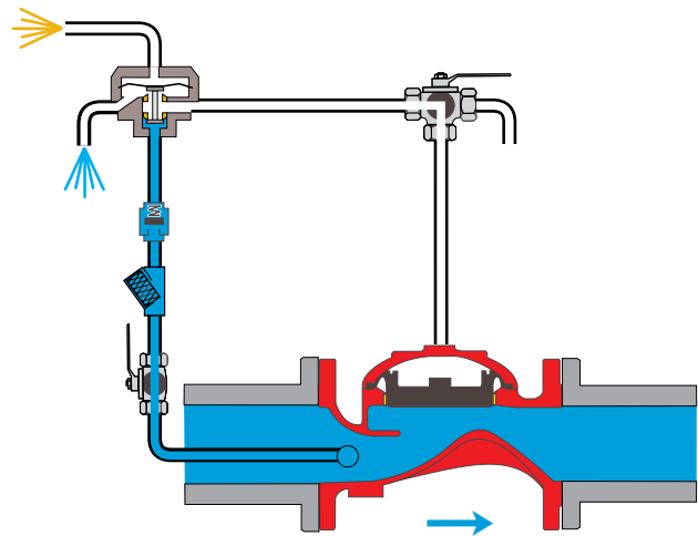
Valve Open (operating condition)
